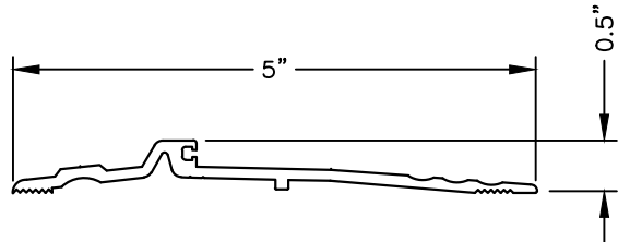
40 THRESHOLD
