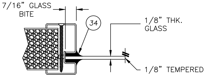
G1 GLAZING DETAIL 9/16" MONOLITHIC GLASS
