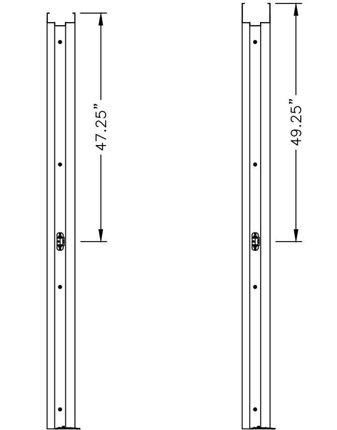
STRIKE PLATE LOCATION 2" HEAD STRIKE PLATE LOCATION 4" HEAD
