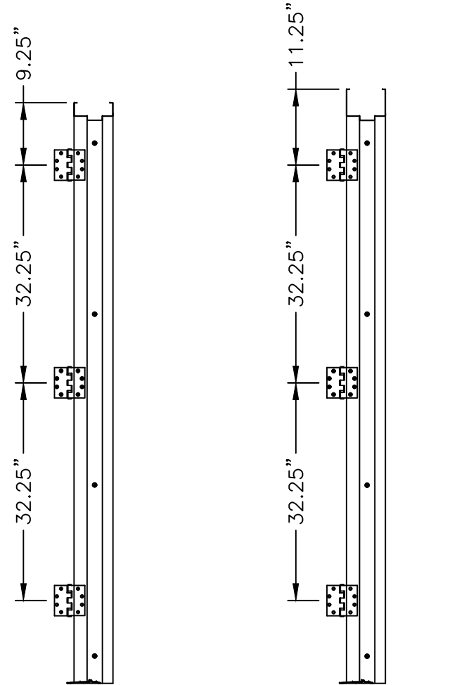
HINGE LOCATIONS 2" HEAD HINGE LOCATIONS 4" HEAD
