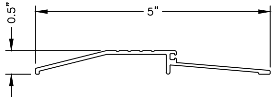
41 THRESHOLD
