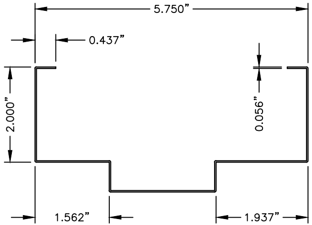
25 FRAME
