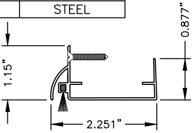
44 SWEEP
