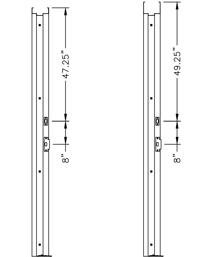
STRIKE PLATE LOCATIONS 2" HEAD STRIKE PLATE LOCATIONS 4" HEAD
